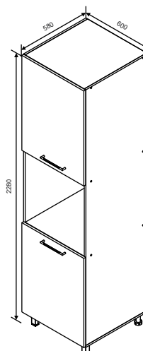
MM 1 Modul Inalt 600
