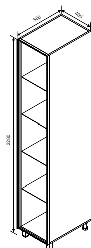
MM 3 Modul Inalt 400
