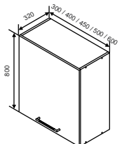
MS 3 Modul superior 300/400/450/500/600
