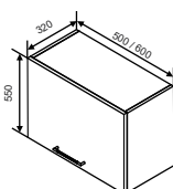
MS 2 Modul superior 500/600
